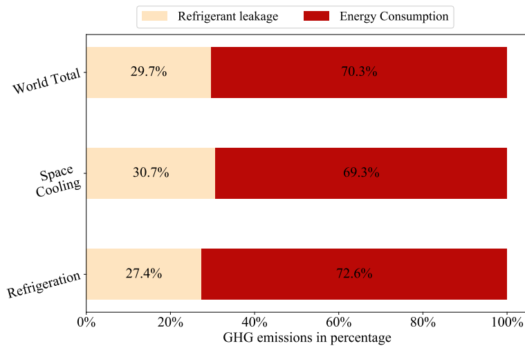
(a) Total Emissions, Space cooling and Refrigeration
