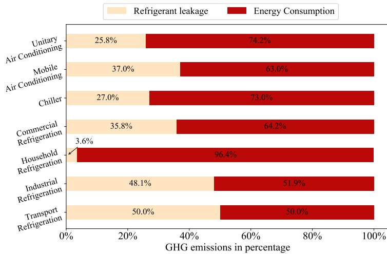
(b) Subcategories of cooling and refrigeration
