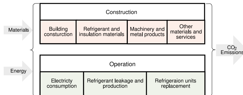
Figure 1: The system boundary of calculating the cold warehouse emissions in China. The calculation of each province is based on this figure and the emissions in Chain are aggregated from each province.
