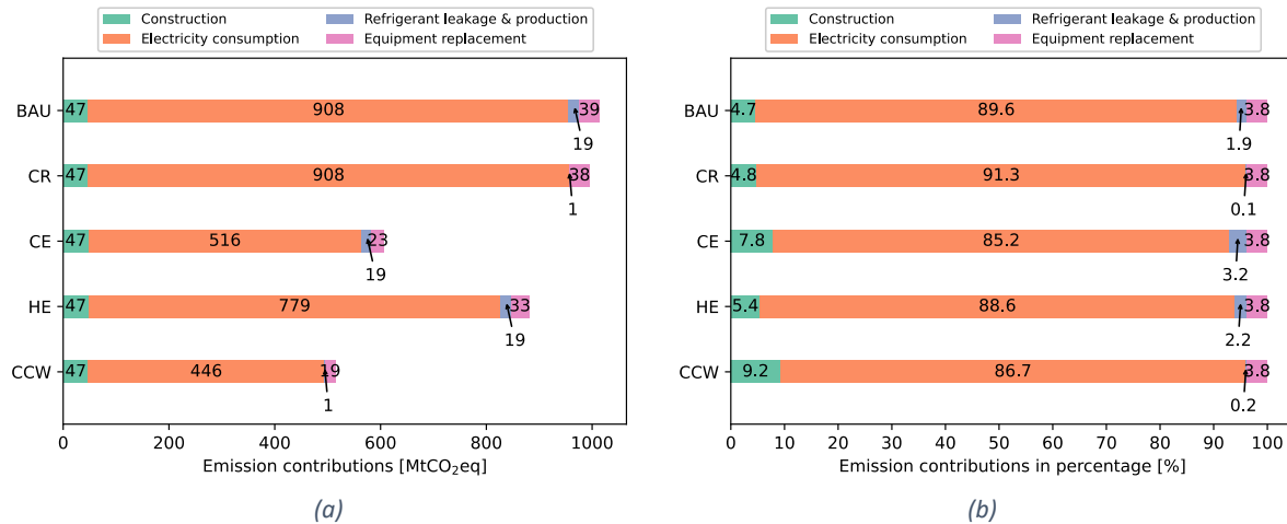
Figure 5: 40-year accumulated emissions break down by emission contributions. Equipment replacement includes those emissions from replacement, reproduction, and retirement. Panel (a) presents the emission contributions in absolute values and Panel (b) present emission contributions in percentage.
