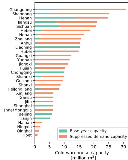
Figure 2: Estimated cold warehouse capacity in 2060. Existing cold warehouse capacity in 2021 (green) and suppressed capacity (orange)
