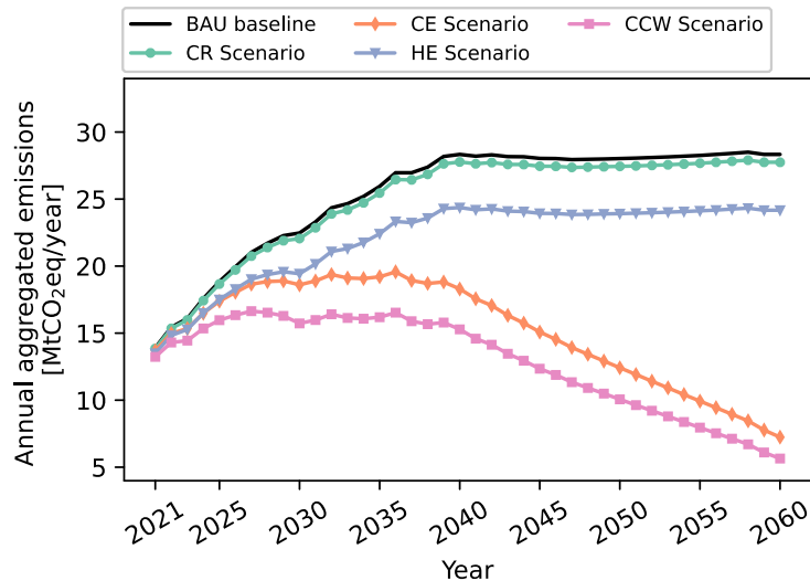
Figure 4: Total estimated annual cold warehouse emissions in China from 2021 to 2060, comparing the emission trend of five scenarios. CR: Cleaner refrigerant; CE: Cleaner electricity; HE: Higher energy efficiency; CCW: Cleaner cold warehouses; BAU: Business-as-usual
