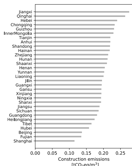
Figure 3: Emissions of building a cold warehouse in each province using EIO analysis
